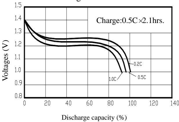
Discharge characteristics
