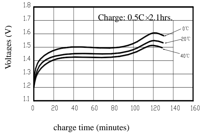
Rapid charge characteristics
