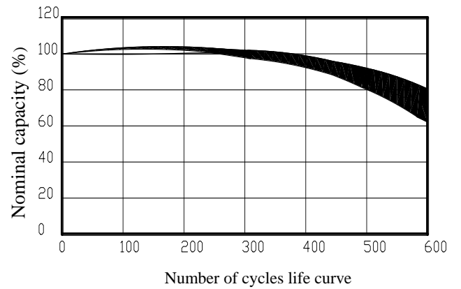
Cycle life characteristics
